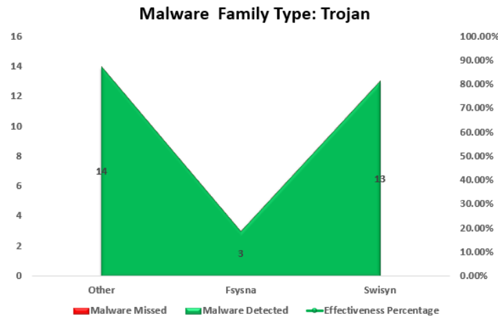
Fig. 14 – Effectiveness against Families of Trojans
