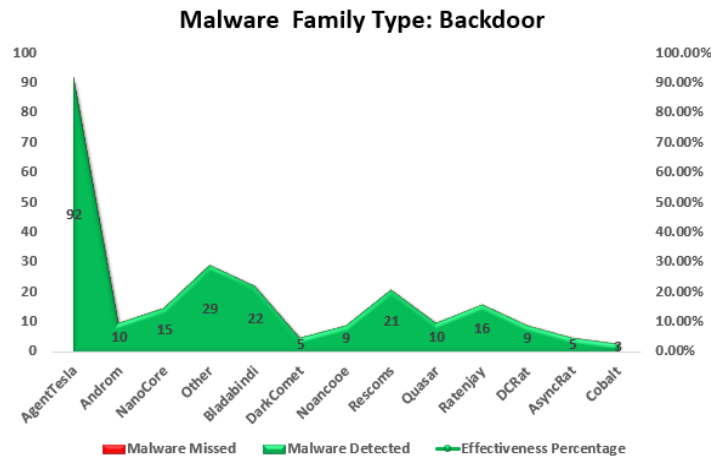
Fig. 16 – Effectiveness against Backdoors
